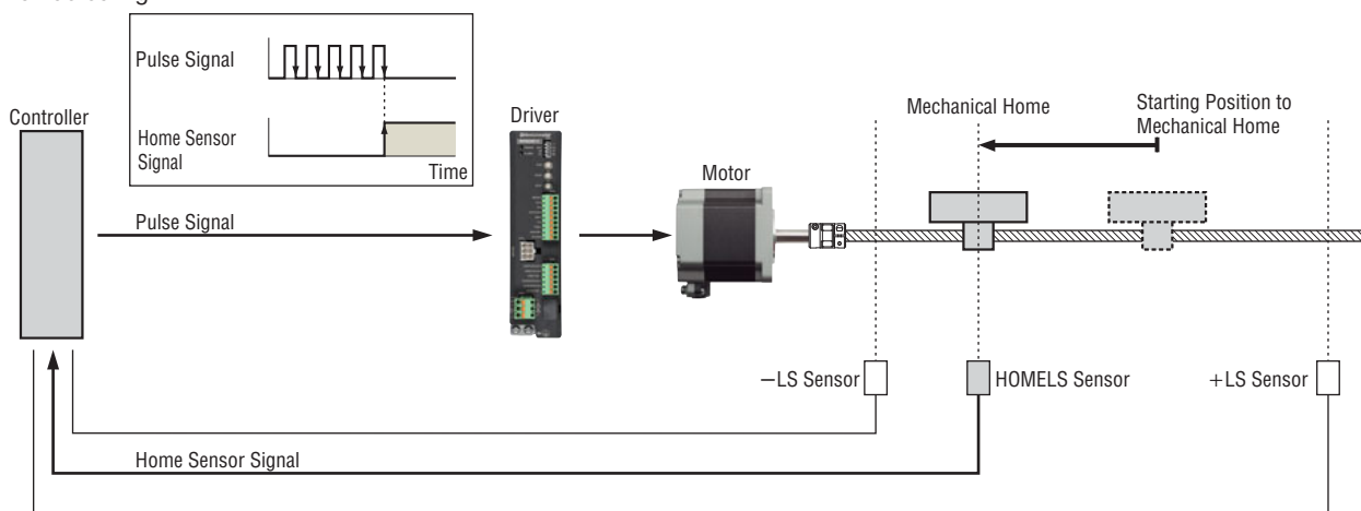
Return to Mechanical Home Operation Using Sensors (3-sensor mode: HOME, CW LS, CCW LS)
