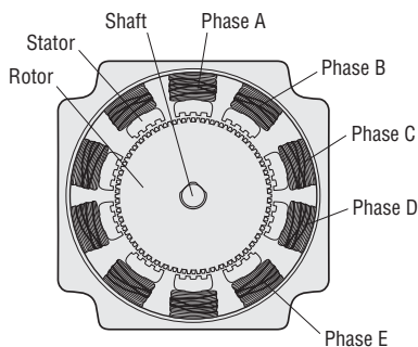
0.72° Stepper Motor Structural Diagram: Cross-Section Perpendicular to Shaft
