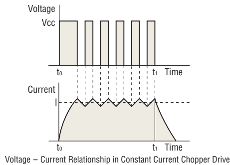
Voltage - Current Relationship in Constant Current Chopper Drive
