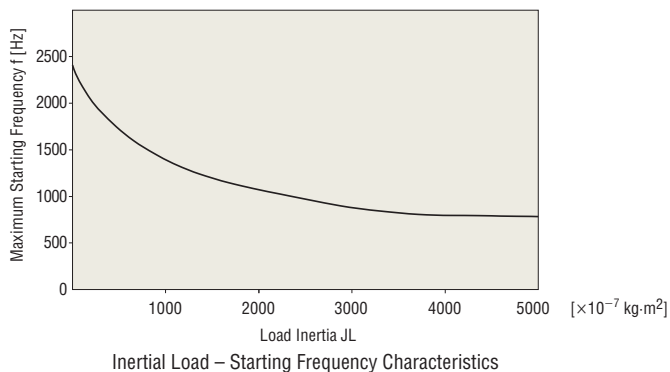
Inertial Load – Starting Frequency Characteristics
