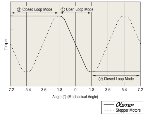
Angle – Torque Characteristics
