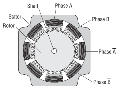
1.8° Stepper Motor Structural Diagram: Cross-Section Perpendicular to Shaft
